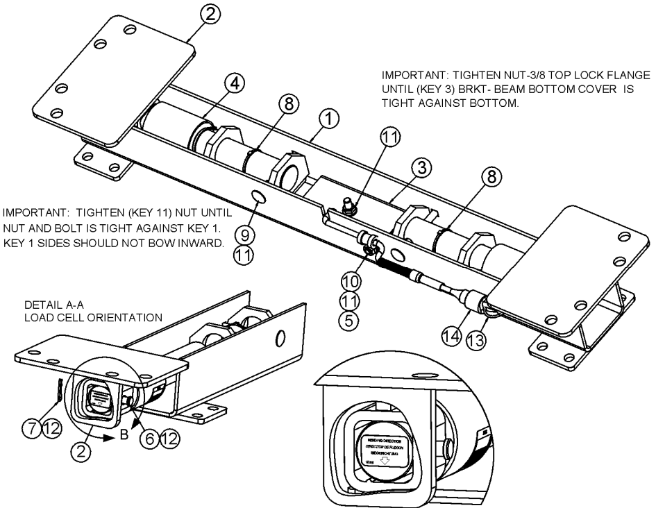
DETAIL B
